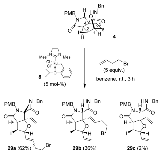
Scheme 8. A control domino metathesis reaction of 4 in the presence of but-3-enyl bromide as a CM substrate.
