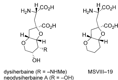
Figure 4. Dysis herbaine congeners [9,10] and the antagonistic analogue MSVIII-19. [41]
