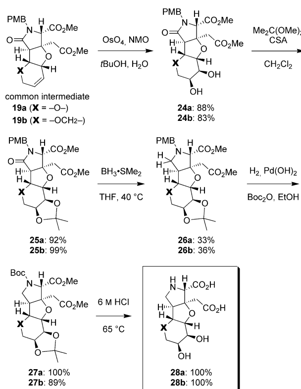
Scheme 7. Synthesis of two glutamate analogues, 28a and 28b , with dihydroxylated ether rings.
