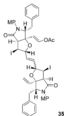
Figure 3. A dimer, 35 , isolated as one of the ROMP products in the domino metathesis of 32 (Table 3, run 1).
