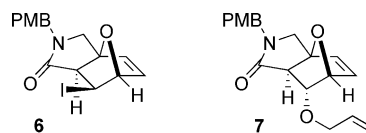
Figure 1. Two 7-oxanorbornenes without amide side chains, used for control metathesis experiments.
