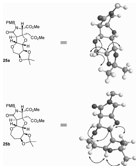
Figure 2. Key NOEs for stereochemical confirmation of compounds 25a and 25b . Plain and dashed arrows indicate NOEs observed at the \beta -side and the \alpha -side of the molecules, respectively. PMB and two methyl esters are omitted for clarity.
