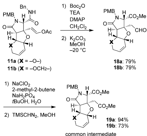
Scheme 5. Synthesis of common intermediates 19a and 19b .
