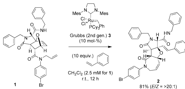
Scheme 1. Our previous demonstration for regioselective domino metathesis of 7-oxanorbornene. [2]
