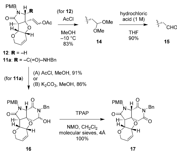
Scheme 4. Failed attempt to construct the glutamate structural unit from 11a .
