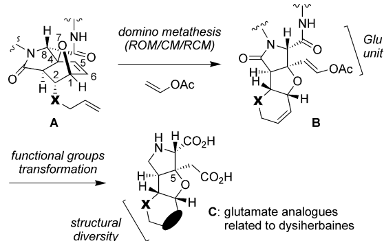
Scheme 2. Our strategy for the synthesis of artificial glutamate analogues by a key domino metathesis reaction in the presence of vinyl acetate.
