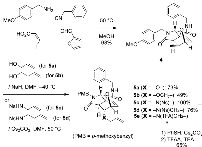
Scheme 3. Tandem Ugi/Diels–Alder reaction followed by introduction of heteroalkenyl groups to synthesize 7-oxanorbornenes as metathesis substrates.
