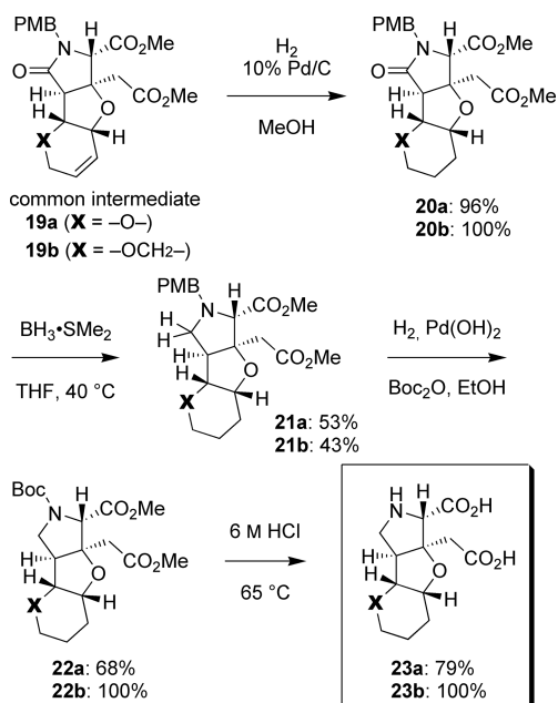
Scheme 6. Synthesis of two glutamate analogues, 23a and 23b , with saturated ether rings.
