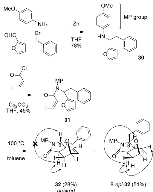
Scheme 9. Preparation of 7-oxanorbornene 32 for control experiments. Arrows on 32 and 8-epi-32 indicate key NOEs for stereochemical assignments.
